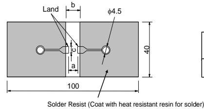
Fig.1 (in mm)
