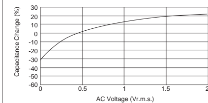
[Example of AC Voltage Characteristics]
