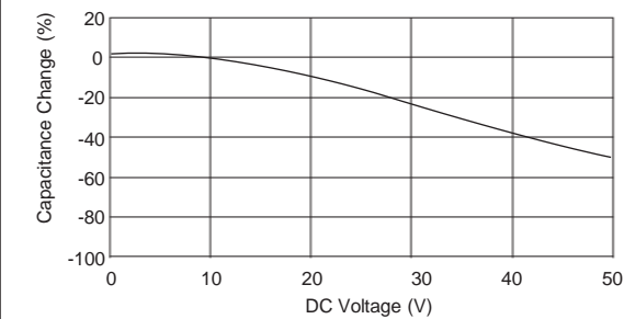
[Example of DC Voltage Characteristics] Sample: X7R(R7) Characteristics 0.1 \mu F, Rated Voltage 50VDC
