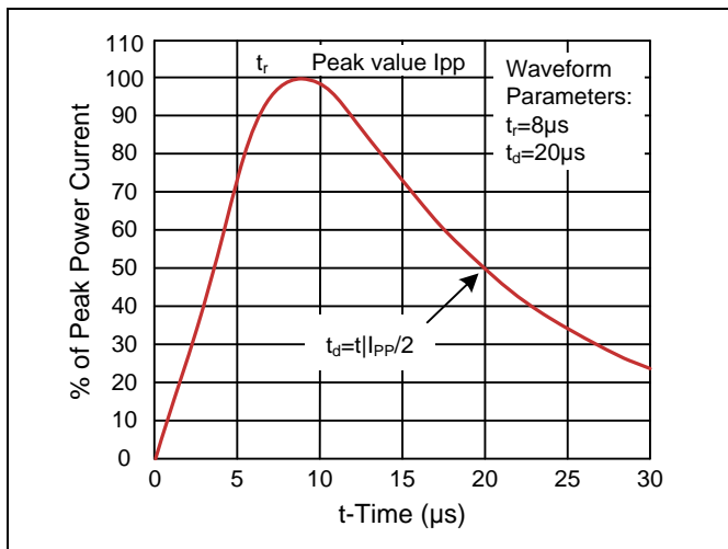
Figure 1. Pulse Waveforms
