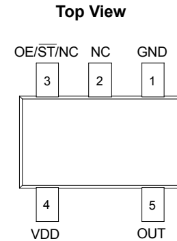
Figure 1. Pin Assignments
