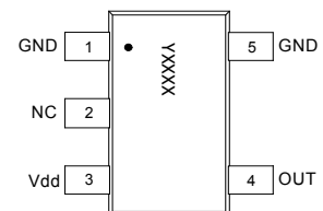
SOT23-5 Package (Top View)
