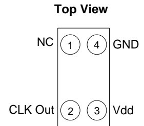
Figure 1. Pin Assignment
