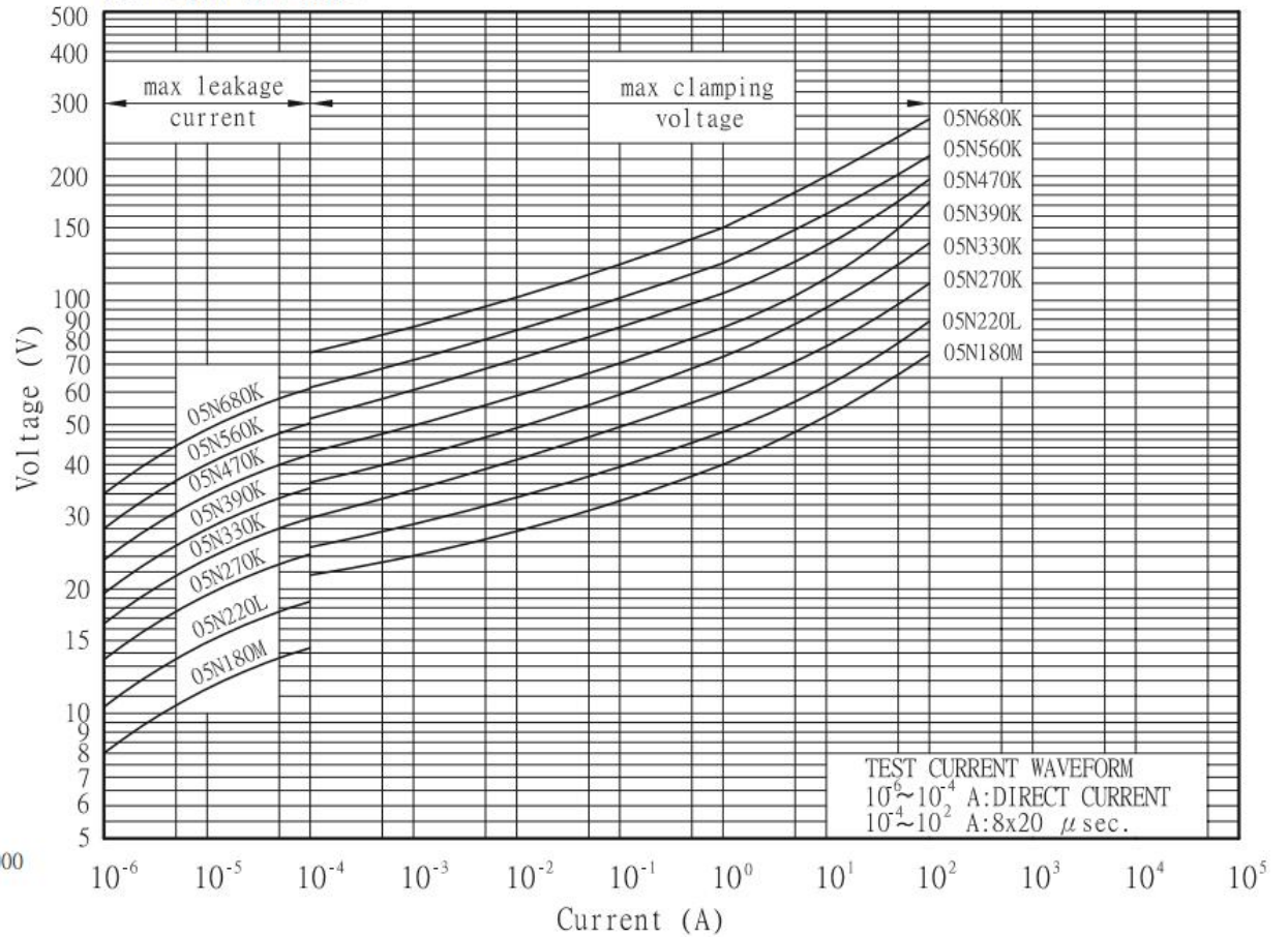
V-I Characteristic Curve-5mm 05N 180M~05N 680K
