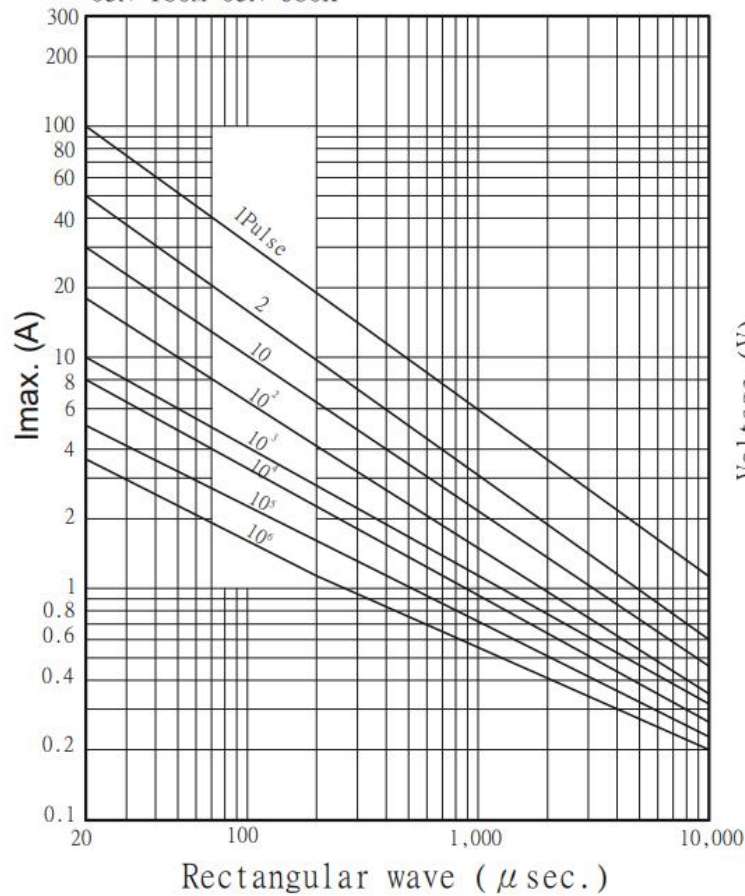
Pulse Life time Ratings-5mm 05N 180M~05N 680K
