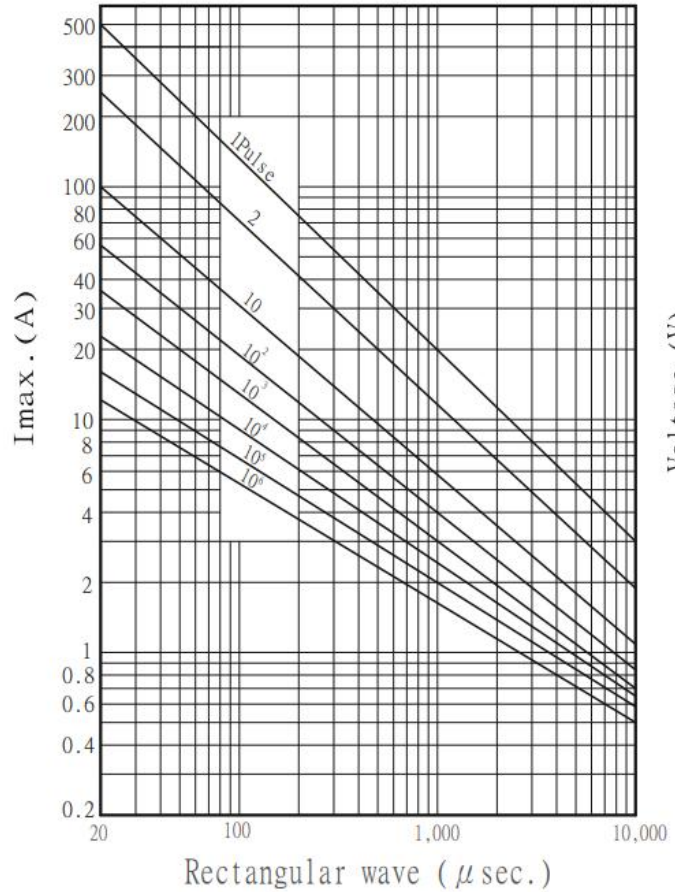
Pulse Life time Ratings -7mm 07S 180M~07 S680K
