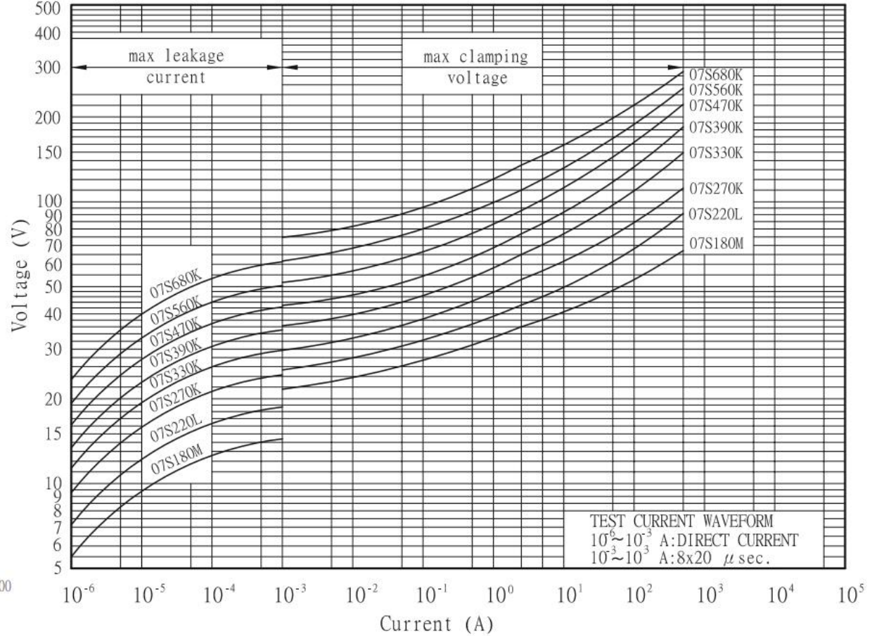
V-I Characteristic Curve -7mm 07S 180M~07 S680K
