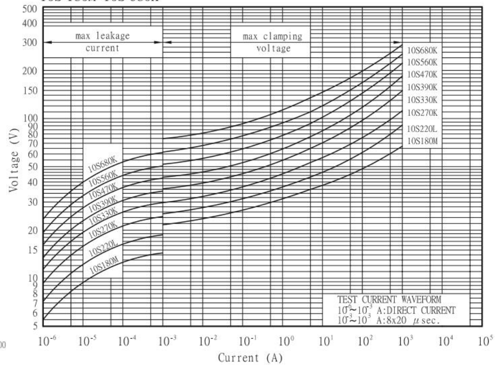
V-I Characteristic Curve-10mm 10S 180M~10S 680K
