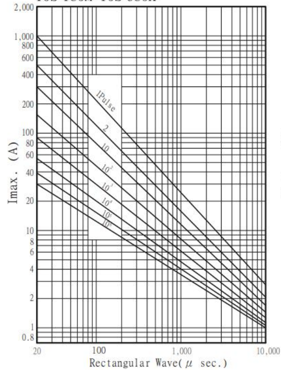
Pulse Life time Ratings-10mm 10S 180M~10S 680K
