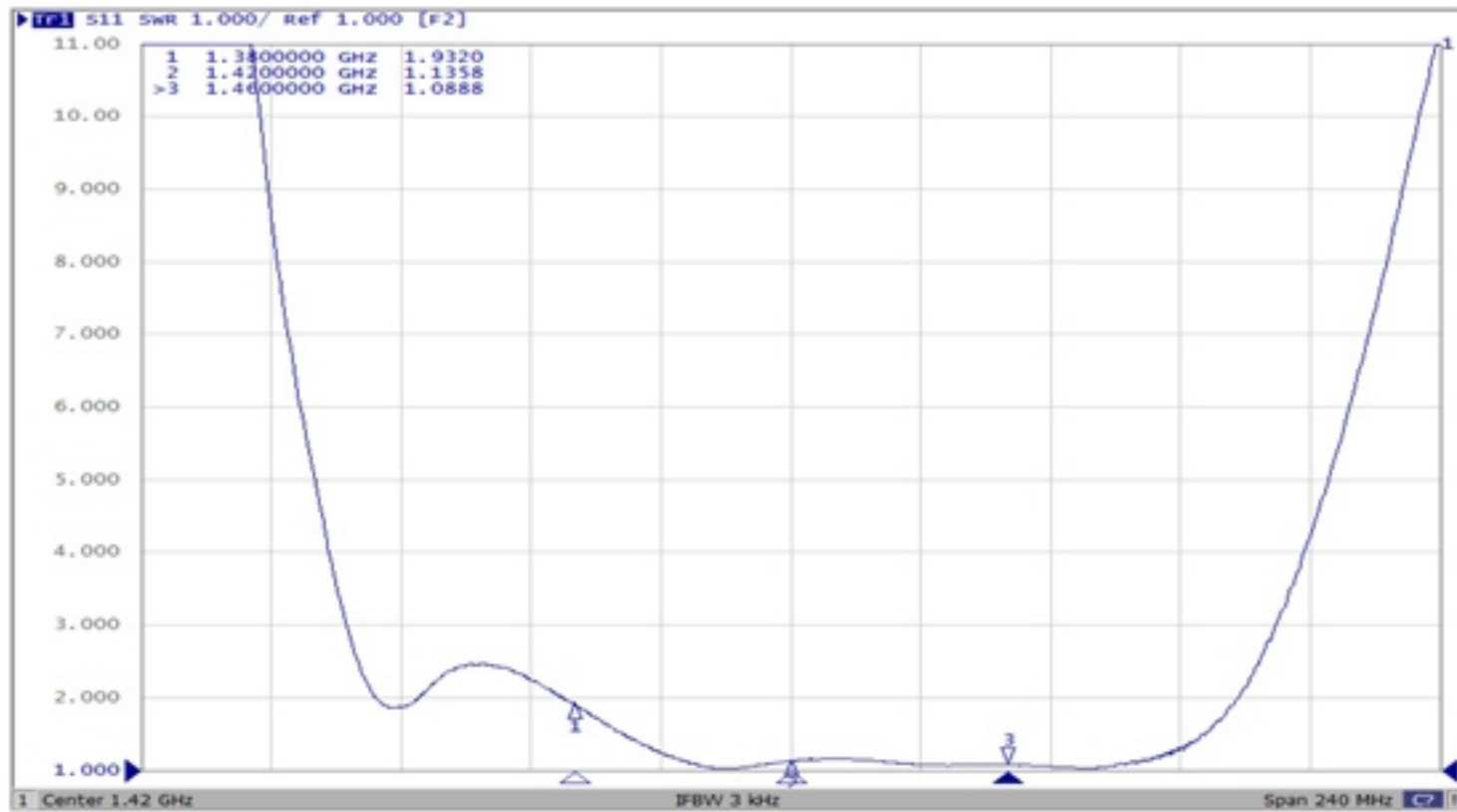
S11
