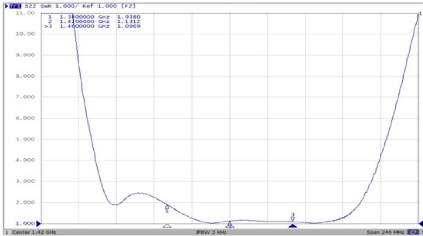
S22
